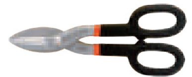
METAL STRAIGHT SHEAR Part No. L. (m/m) Capacity 1500303 180 0.8mm 1500304 200 0.8mm 1500305 260 0.8mm 1500306 350 0.8mm
